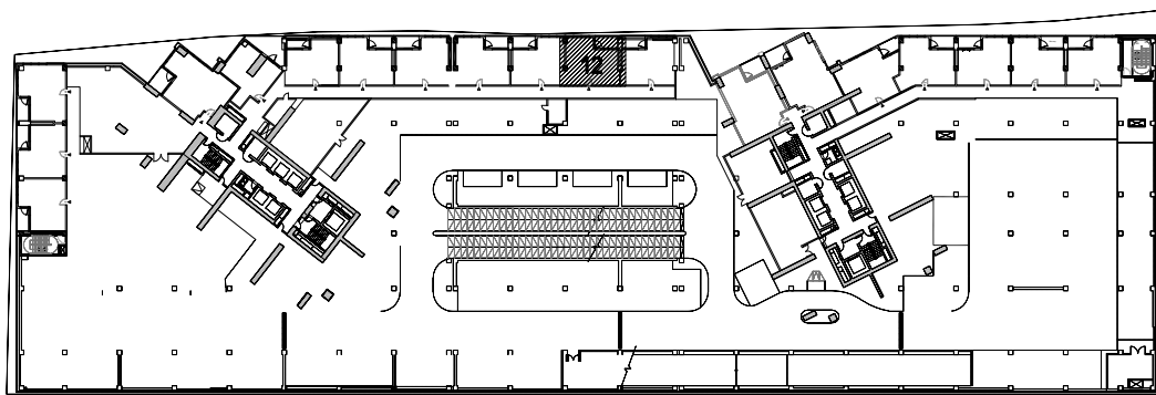
PODIUM LEVEL 2
